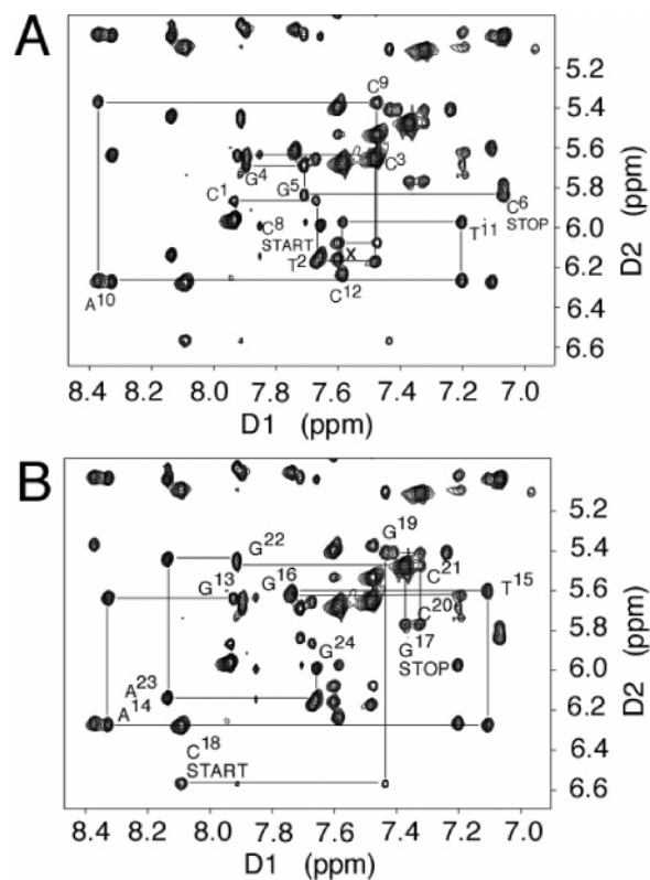
Figure 1. Aromatic-anomeric proton region of the 800.13 MHz NOESY spectrum for the Nar1IQ3 duplex at 15 °C at 250 ms mixing time, showing sequential NOE connectivity. (A) Nucleotides C 1 \rightarrow C 12 of the modified strand. (B) Nucleotides G 13 \rightarrow G 24 of the complementary strand.
