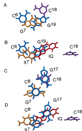
Figure 11. Base stacking of the Nar1IQ3 and the unmodified duplexes. (A) Unmodified duplex. Stacking of C 6 ·G 19 and G 7 ·C 18 . (B) Nar1IQ3 duplex. Stacking of C 6 ·G 19 and X 7 ·C 18 . (C) Unmodified duplex. Stacking of G 7 ·C 18 and C 8 ·G 17 . (D) Nar1IQ3 duplex. Stacking of X 7 ·C 18 and C 8 ·G 17 .
