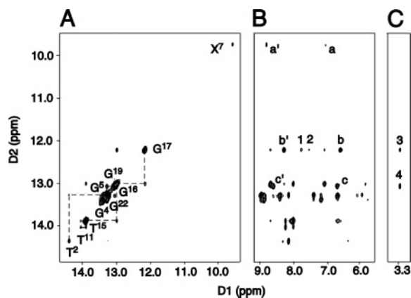
Figure 2. (A) Sequential NOE connectivity for the imino protons of base pairs T 2 ·A 23 → T 11 ·A 14 for the Nar1IQ3 duplex at 5 °C. The labels represent the imino proton of the designated base. (B) NOE connectivity between the imino protons and the base and amino protons. The cross-peaks involving the imino protons are labeled as: a', a, X 7 N1H → X 7 NH 2 -2b, e; b', b, G 17 N1H → C 8 NH 2 -4b, e; c' and c, G 19 N1H → C 6 NH 2 -4b, e; 1, G 17 N1H → X 7 H4A; 2, G 17 N1H → X 7 H5A. (C) NOE connectivity between the imino and the IQ methyl protons. The IQ-DNA cross-peaks labeled are as: 3, G 17 N1H → X 7 CH 3 ; and 4, G 19 N1H → X 7 CH 3 .
