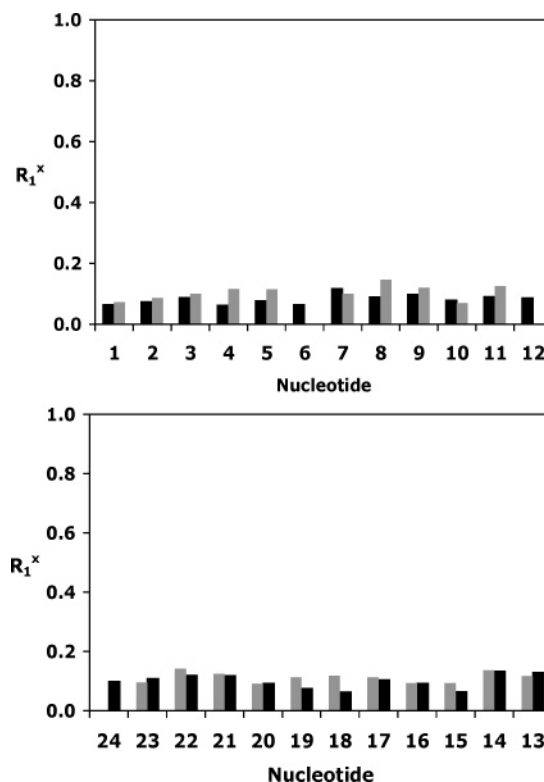
Figure 9. Sixth root residuals for NOE intensities of the Nar1IQ3 duplex. (Top) Nucleotides C 1 → C 12 . (Bottom) Nucleotides G 13 → G 24 . Dark bars represent intranucleotide values; light bars represent internucleotide values.
