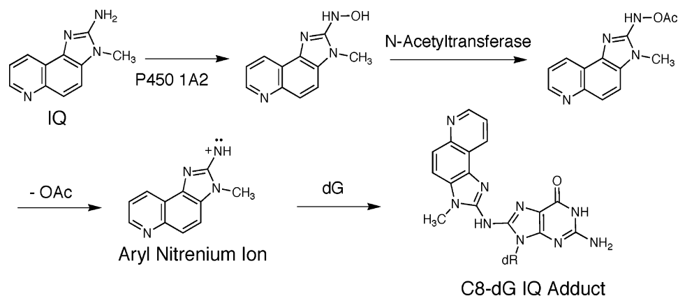
Chart 1. Metabolic Activation of IQ
