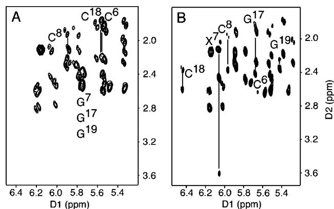
Figure 5. Expanded COSY spectra at 15 °C, establishing connectivity between the H1' and H2' , H2'' protons. The H2' and H2'' protons of the nucleotides adjacent to the lesion site are labeled. (A) Unmodified duplex. (B) Nar1IQ3 duplex.
