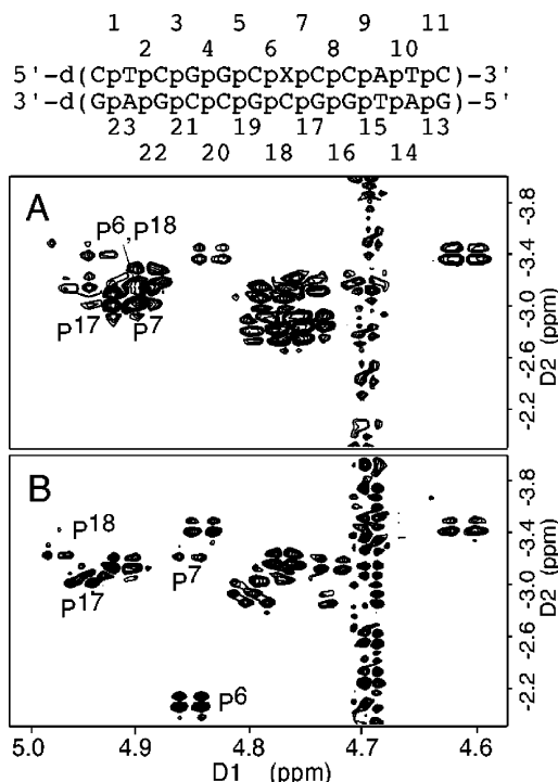
Figure 6. H3' regions of nonselective excitation ^{31}P - ^1H HMBC spectra of the unmodified (upper) and the Nar1IQ3 duplexes (lower). Both spectra were collected at 15 °C.
