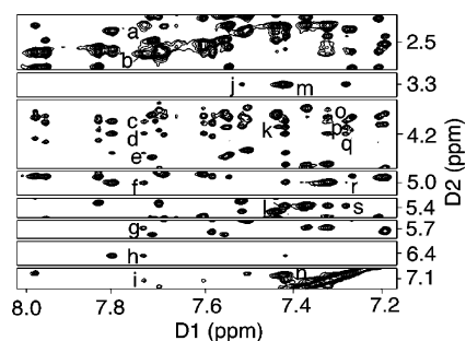
Figure 4. NOE cross-peaks between nonexchangeable protons of DNA and IQ protons in the Nar1IQ3 duplex. (a–i) G^{17} H2' , G^{17} H2'' , C^{18} H5' , H4' , H5'' , H3' , G^{17} H1' , C^{18} H1' , and G^{17} H8 \rightarrow IQ H9A ; (j) C^8 H6 \rightarrow IQ CH_3 ; (k–l) G^{19} H5' and G^{19} H1' \rightarrow IQ H4A ; (m–n) G^{19} H8 \rightarrow IQ CH_3 and H5A ; (o–s) G^{19} H5'' , G^{19} H5' , C^{18} H4' , C^{18} H3' , and G^{19} H1' \rightarrow IQ H5A , respectively.
