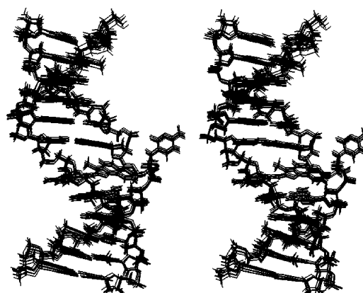
Figure 8. Stereoview of 10 superimposed structures emergent from randomly seeded rMD calculations on the Nar1IQ3 duplex.
